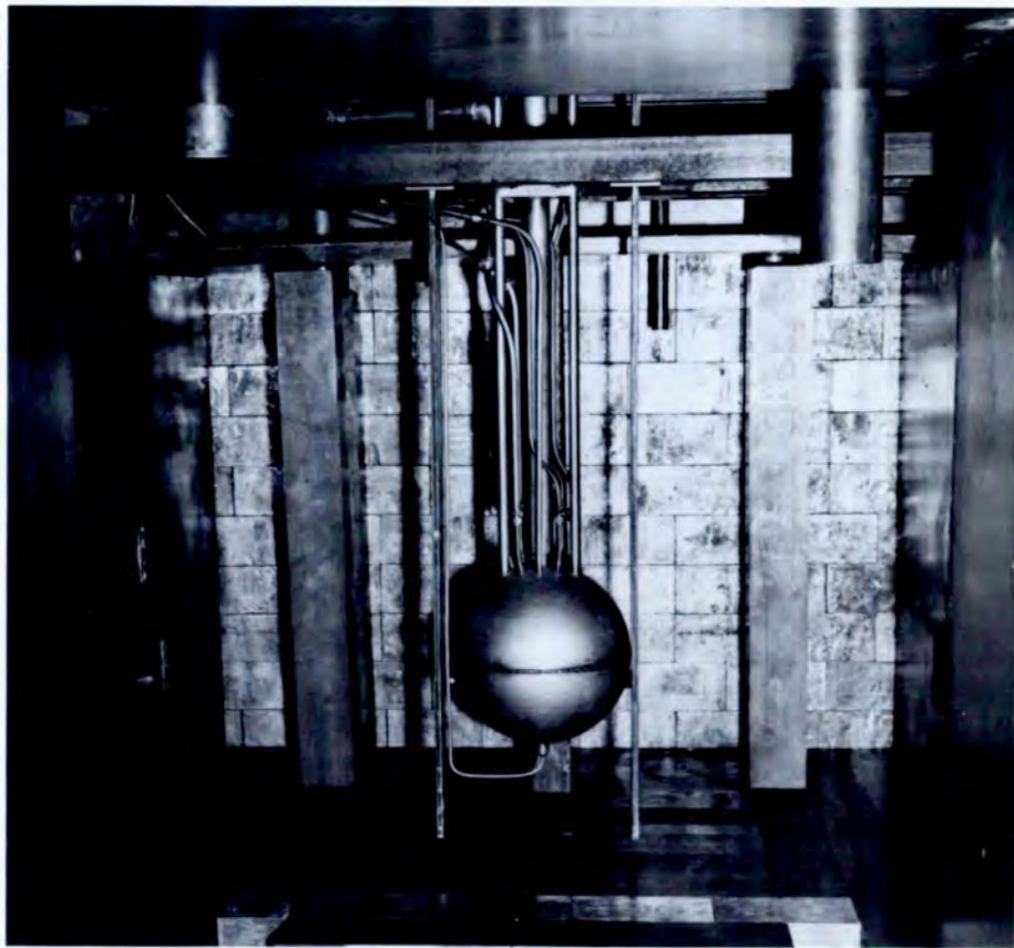
Fig. 3. The SUPO sphere prior to installation of the surrounding graphite reflector. The plates tangent to the sphere are control-rod sheaths. The tube leaving the bottom of the sphere is for addition or removal of fuel solution.
